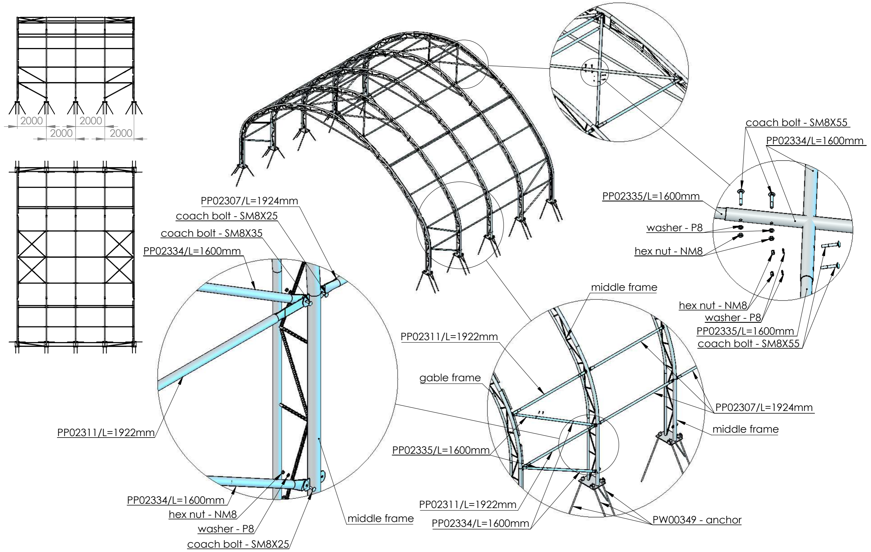
mounting instruction - layout of struts in hall
